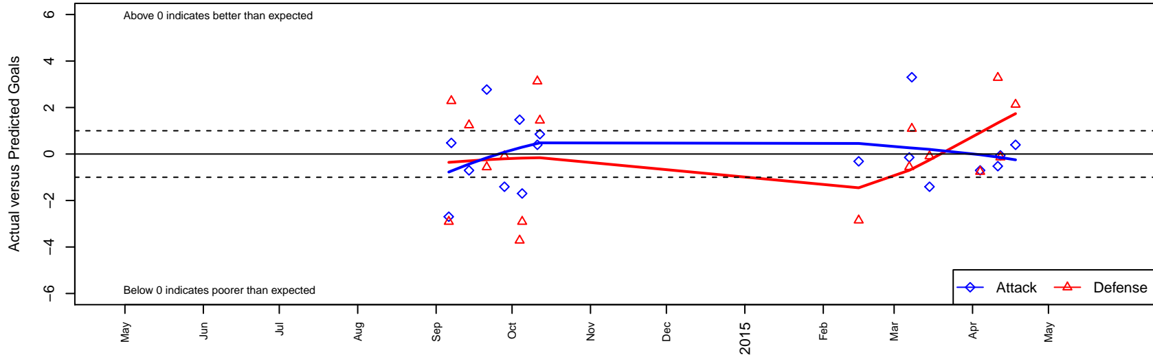
BSC Newberg Vapor B02 Dots are actual minus expected GF (blue circles) and GA (red triangles). Blue line is smoothed change in attack strength. Red is smoothed change in defense strength.
